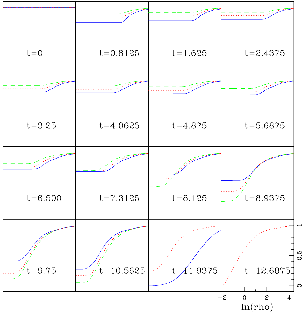
Figure 8.2 — Semilog plot of \alpha(t, \rho) for three initial amplitudes. The weaker initial amplitude (dashed) collapses faster and is the first to approach zero, indicating the formation of a black string.
